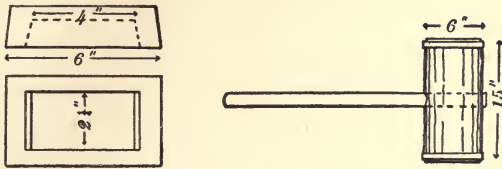
FIG. 15.—DRIVING-CAP AND MAUL.
